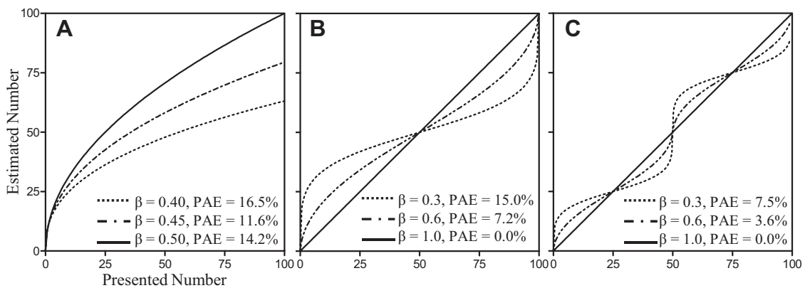
Figure 1. Predictions of the proportion-judgment account, as applied to a typical number-line task. A depicts a one-parameter unbounded power function (with the scaling factor, \alpha , fixed at 10). B and C depict one- and two-cycle versions of the proportional power model, respectively. The two-cycle version of the model depicts the predicted estimation pattern for observers who use the midpoint of the number line as a reference point. PAE = percent absolute error.
