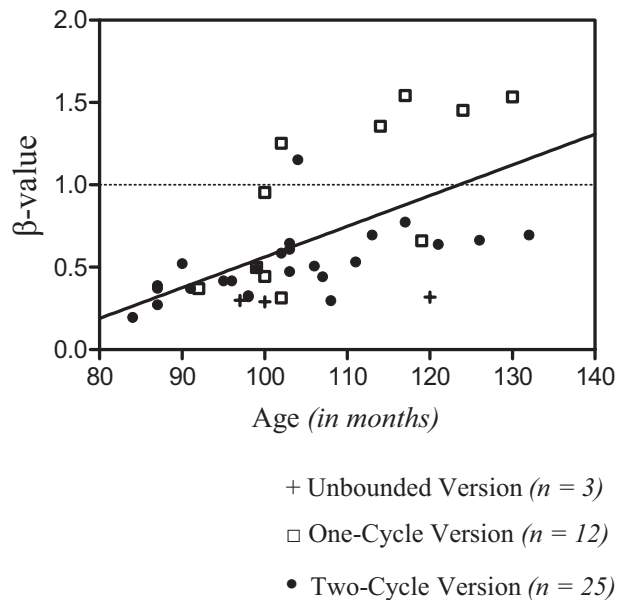
Figure 5. Values of the \beta parameter corresponding to the estimates of each child whose performance is best predicted by the proportion-judgment account on the 0–1000 number-line task ( n = 40 ).
